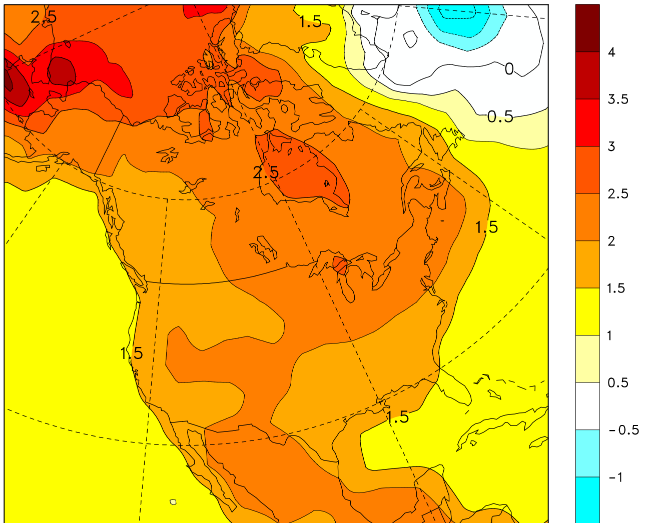
Surface Air Temp, C, change, SRESB1/T47 ANN 2081-2100 vs 1981-2000
