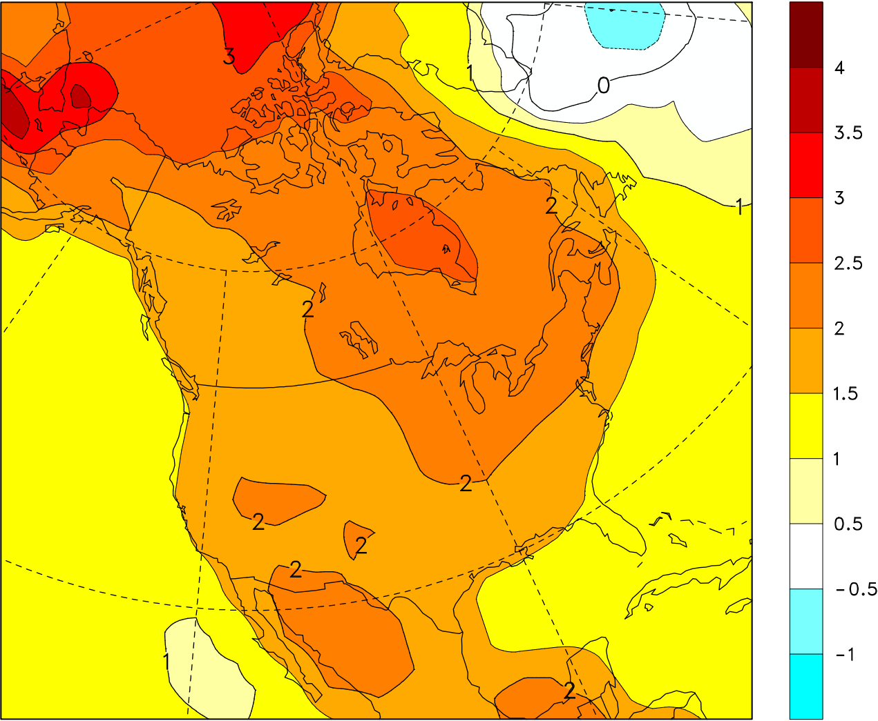
Surface Air Temp, C, change, SRESA1B/T47 ANN 2041-2060 vs 1981-2000
