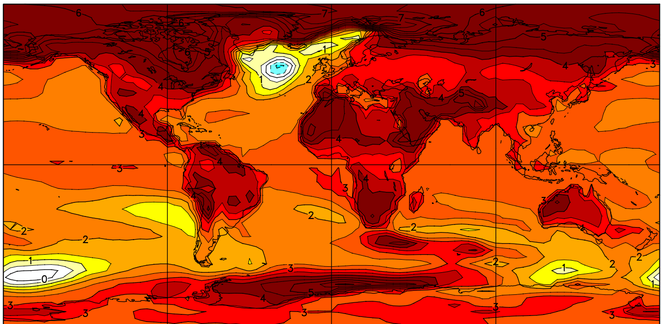
Surface Air Temp, C, change, SRESA1B/T47 ANN 2081-2100 vs 1951-1980
