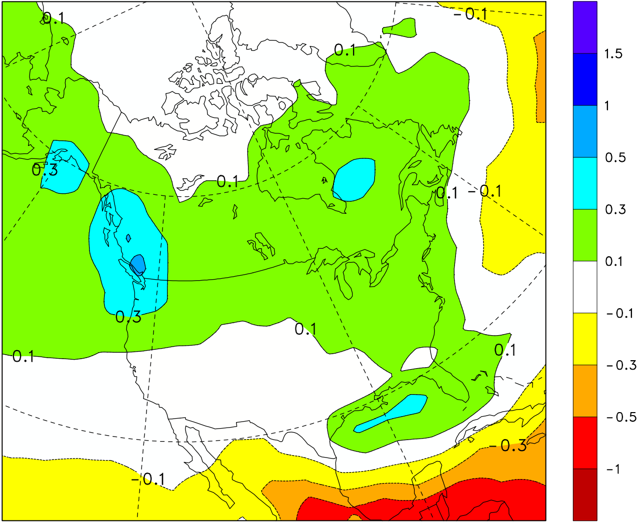
Precipitation, mm/day, change, SRESB1/T47 ANN 2081-2100 vs 1981-2000
