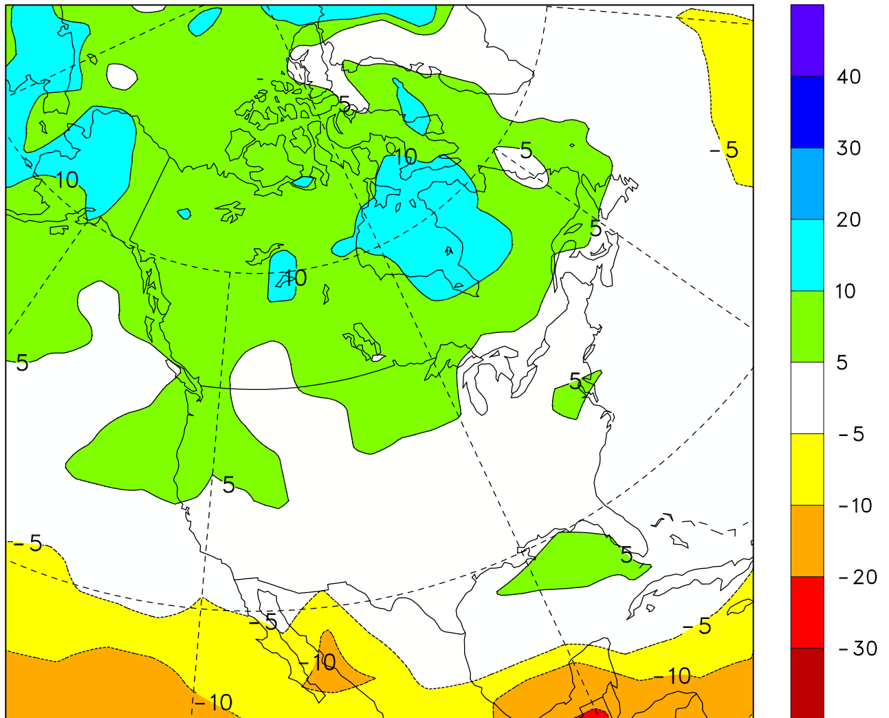
Precipitation, %, change, SRESB1/T47 ANN 2041-2060 vs 1981-2000
