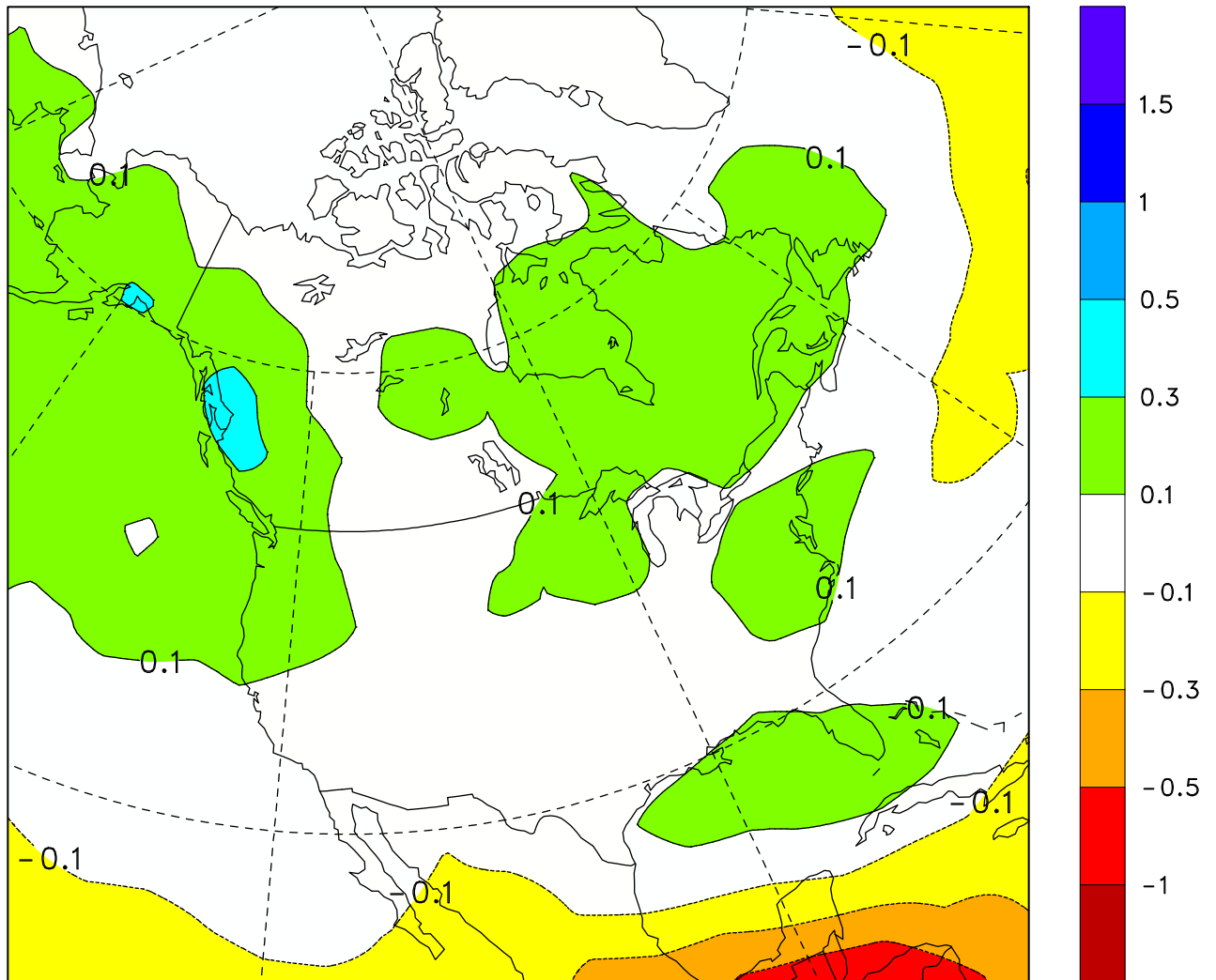
Precipitation, mm/day, change, SRESB1/T47 ANN 2041-2060 vs 1981-2000
