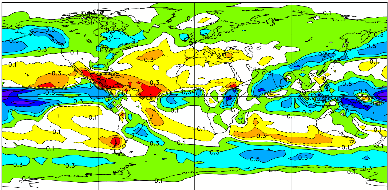
Precipitation, mm/day, change, SRESA1B/T47 ANN 2081-2100 vs 1981-2000
