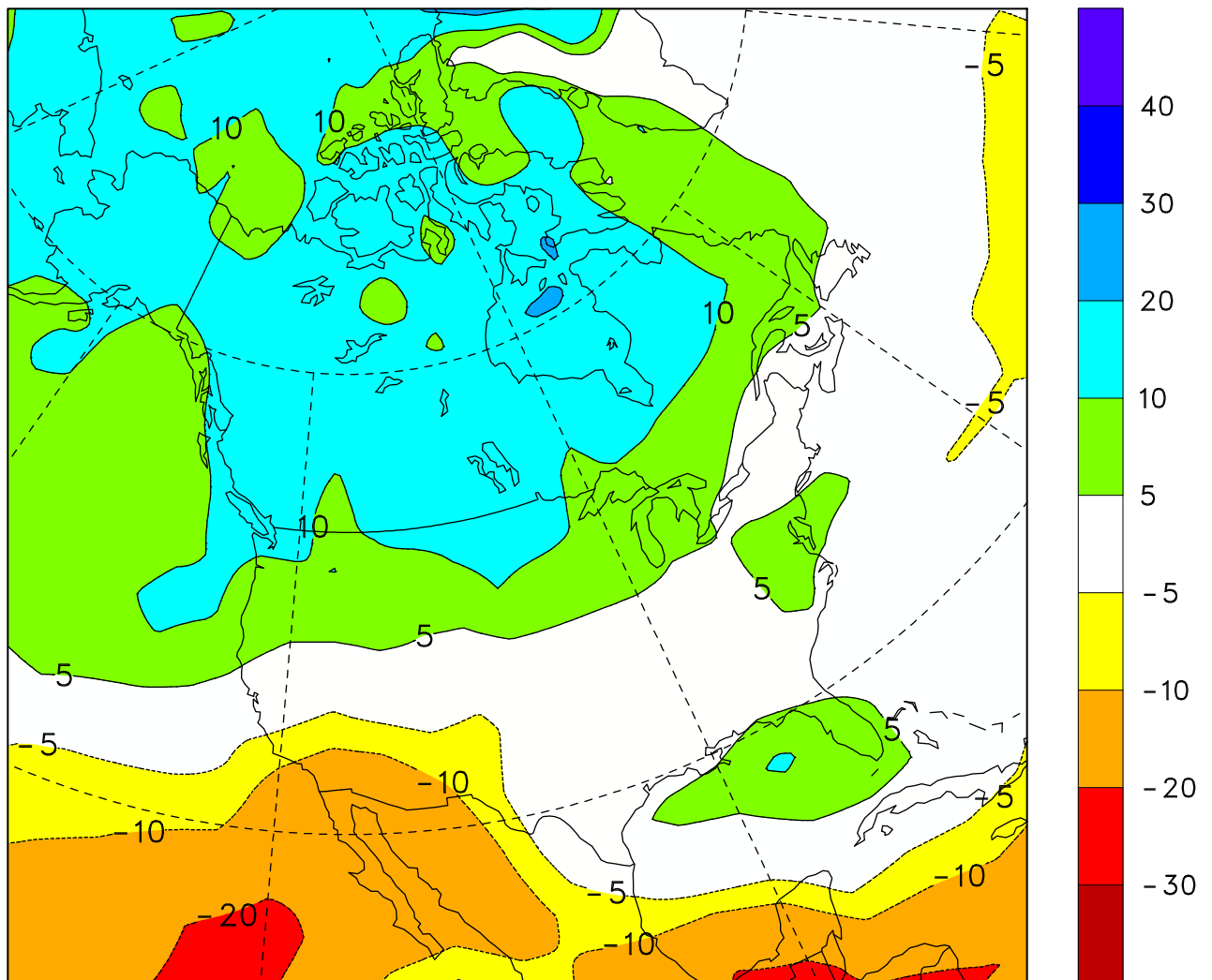
Precipitation, %, change, SRESA1B/T47 ANN 2041-2060 vs 1981-2000
