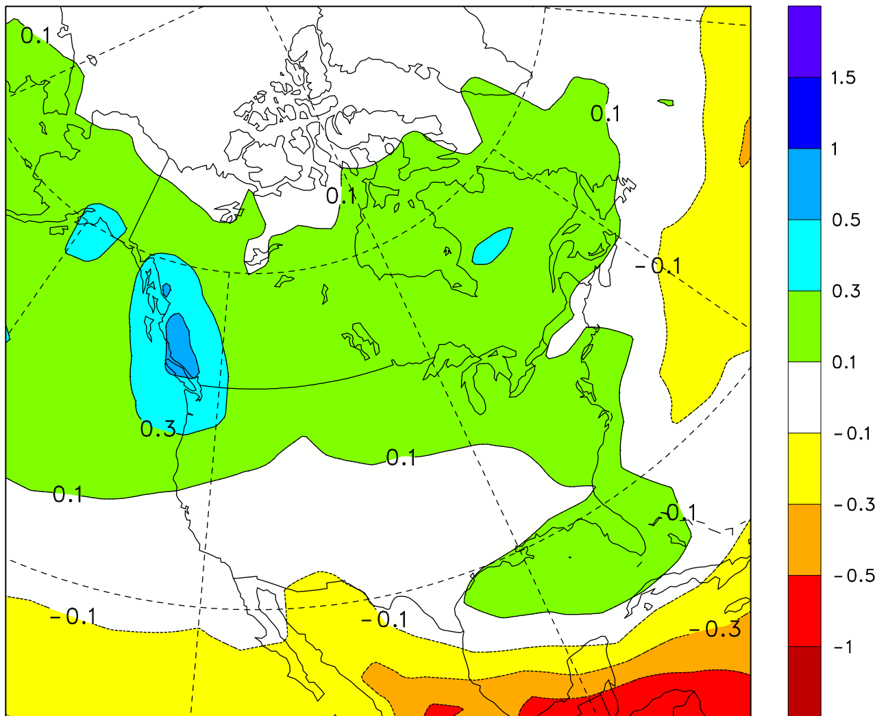
Precipitation, mm/day, change, SRESA1B/T47 ANN 2041-2060 vs 1981-2000
